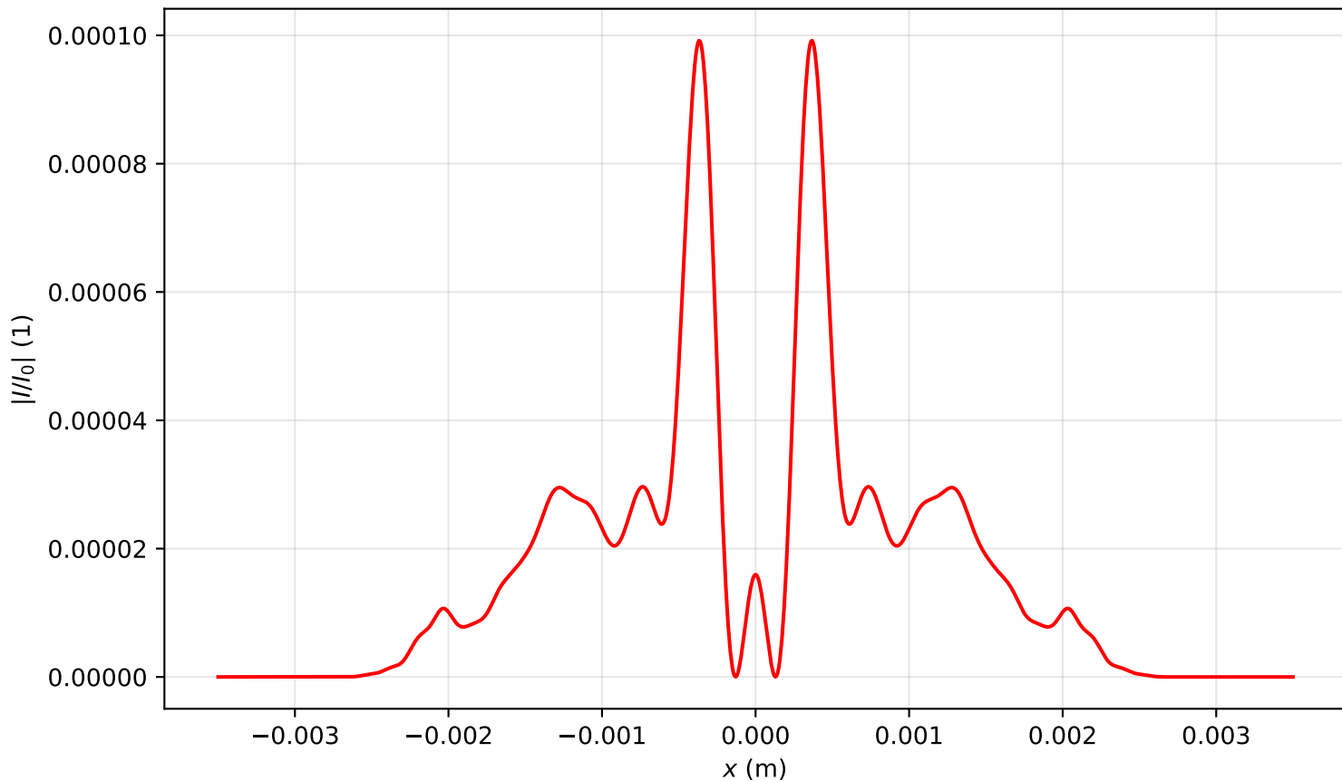
Intensity profile I(x, y = 0, z = 1.353)/I_0 , P_{in}=9.0P_{cr} , artificial time
